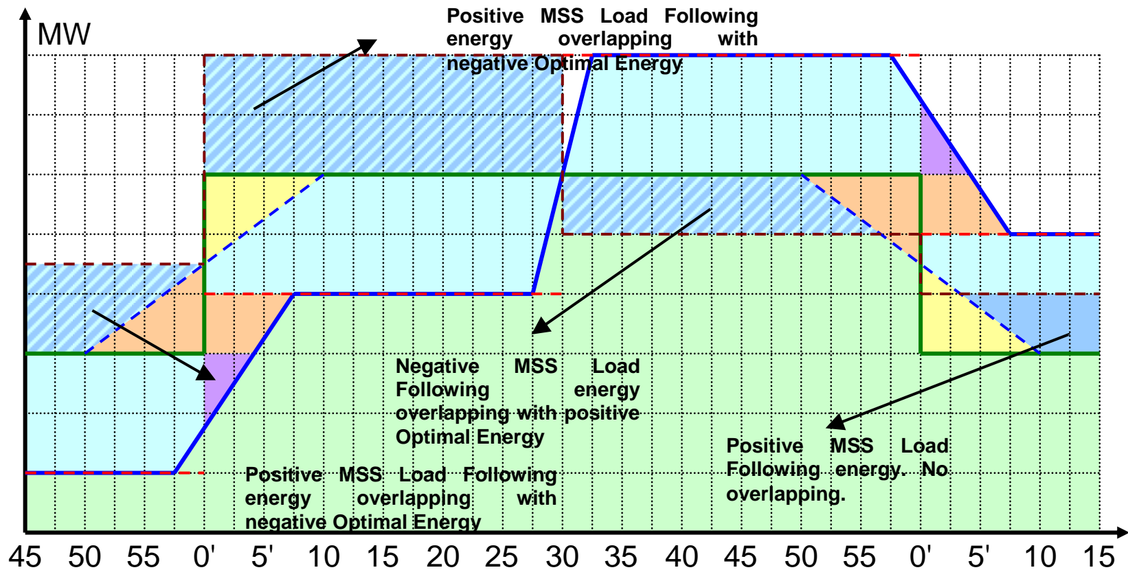
Exhibit C-19: MSS Load Following Energy (Economic Dispatch with MSSLF case 2)
