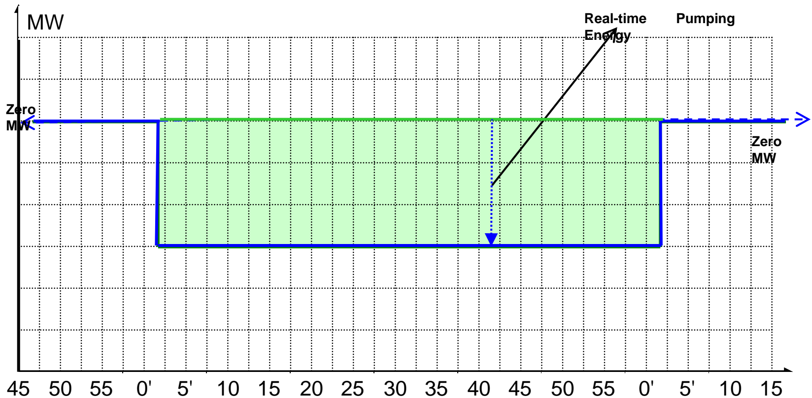
Exhibit C-13: Negative Real-time Pumping Energy
