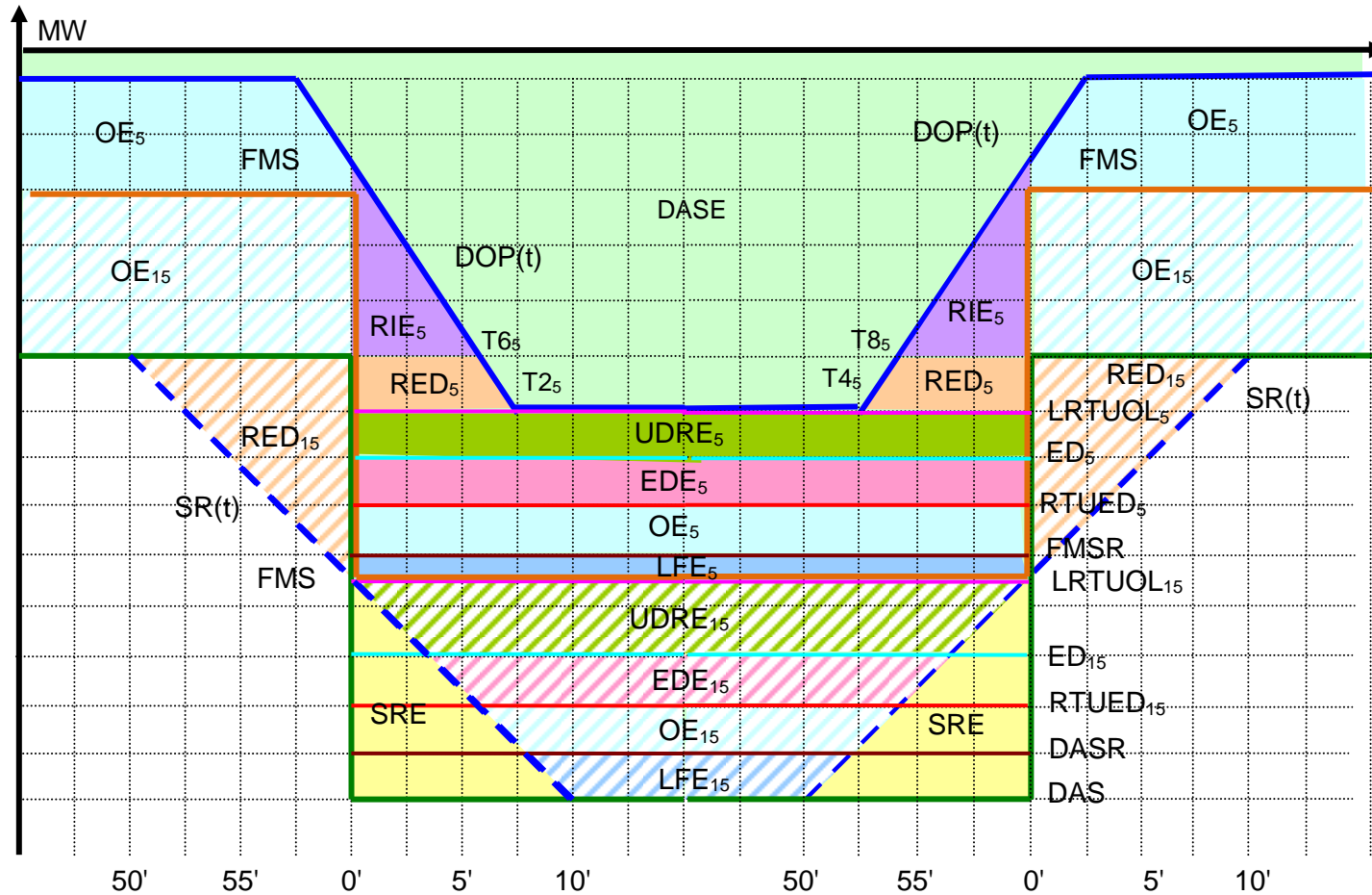
Figure 5h Instructed Imbalance Energy Stack for a NGR. Load side, RTD dispatch greater than DA schedule.
