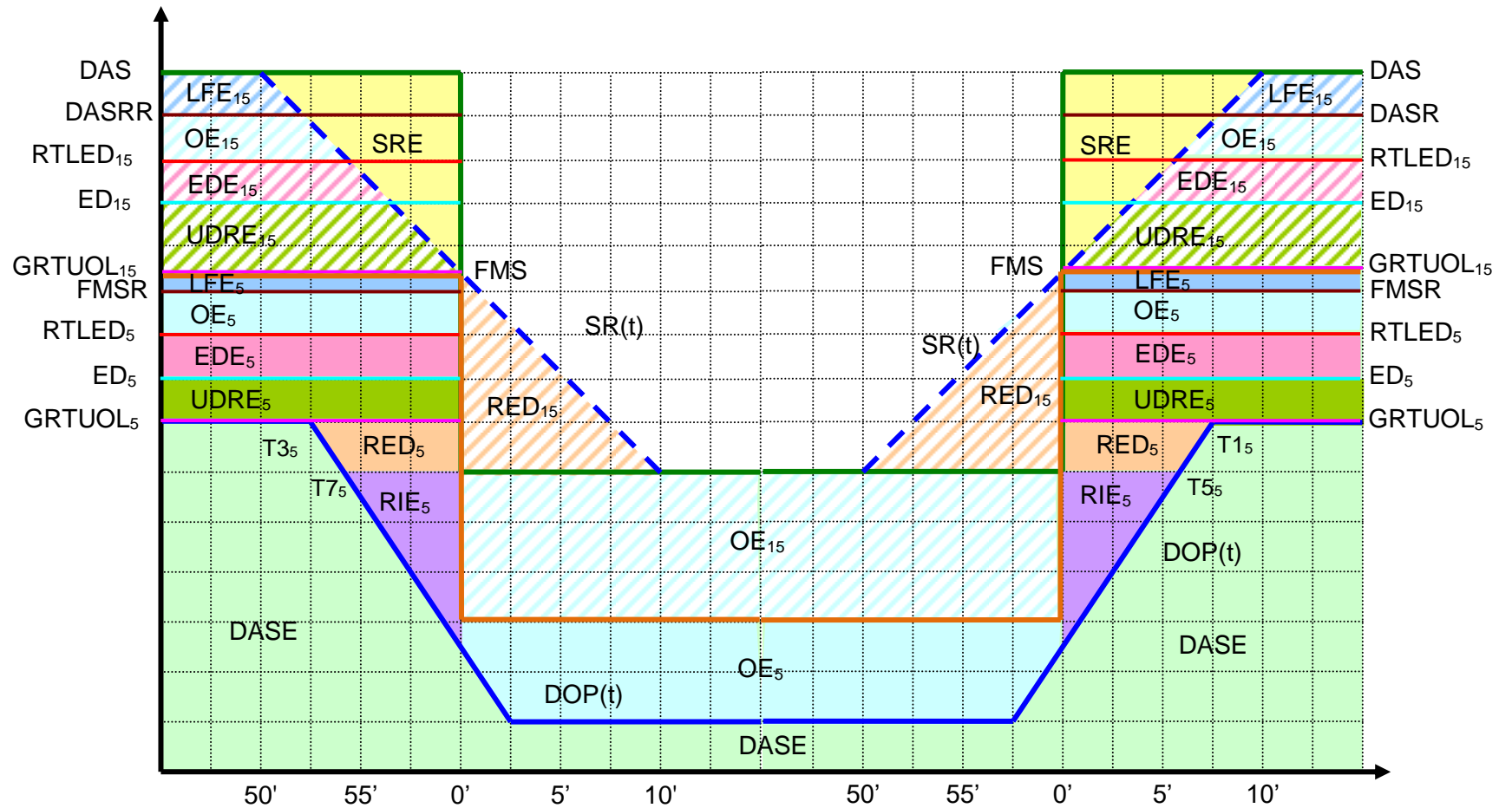
Figure 5g Instructed Imbalance Energy Stack for a NGR. Generation side, RTD dispatch less than DA schedule.
