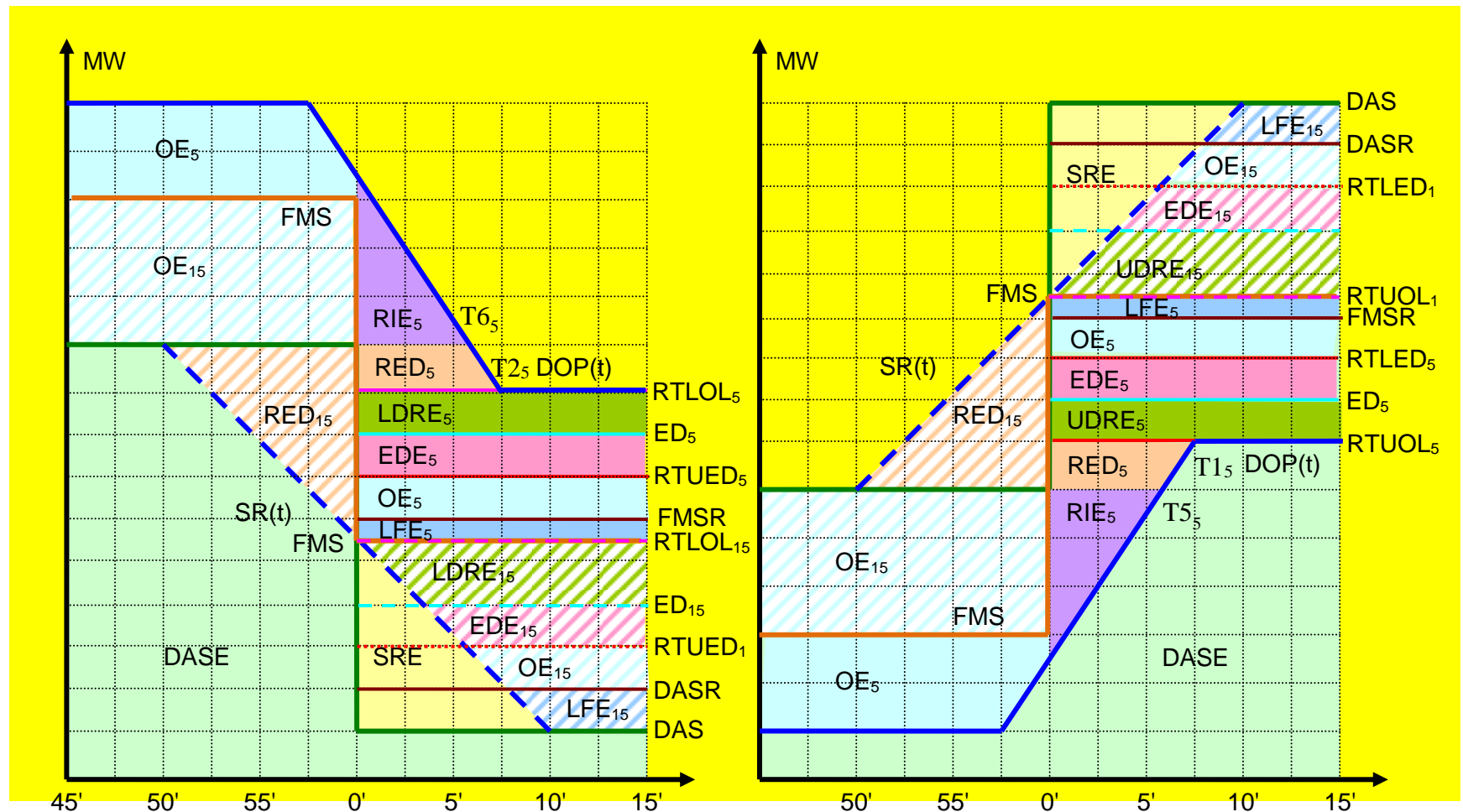
Figure 5a. Instructed imbalance Energy Stack – generation side
