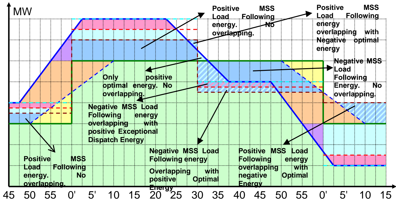
Exhibit C-20: MSS Load Following Energy (D-18 with Exceptional Dispatch)
