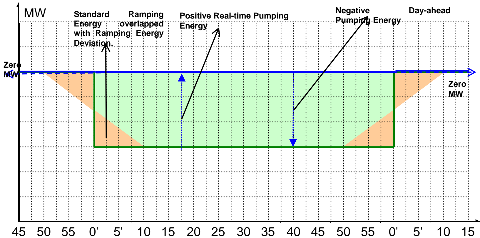
Exhibit C-12: Positive Real-time Pumping Energy
