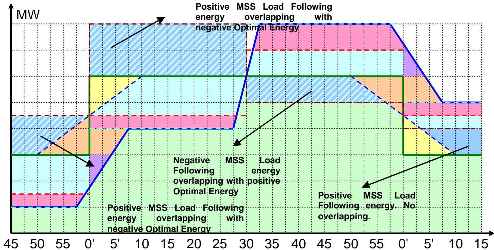
Exhibit C-21: MSS Load Following Energy (D-19 with Exceptional Dispatch)
