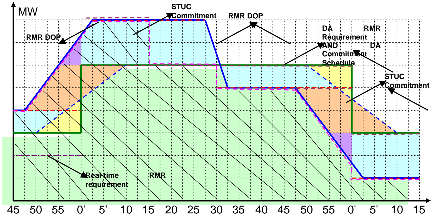
Exhibit C-22: "RMR DOP" curve calculation and RMR energy
