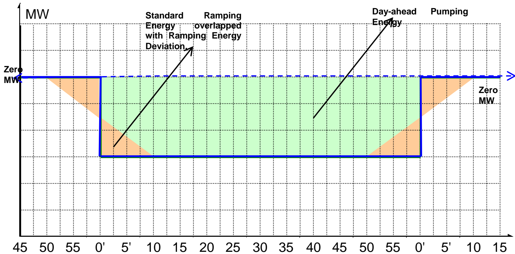
Exhibit C-11: Day-ahead Pumping Energy
