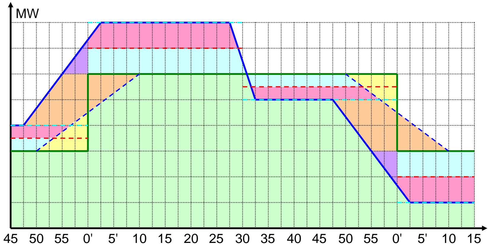
Exhibit C-9 shows an Exceptional Dispatch that generates a DOP curve ramping first up towards the current hour however below Day-Ahead Schedule, further ramp up above the Day-Ahead Schedule in the middle of hour, then ramp further down but above the Day-Ahead Schedule in the following hour. This dispatch pattern results in the following Expected Energy:
